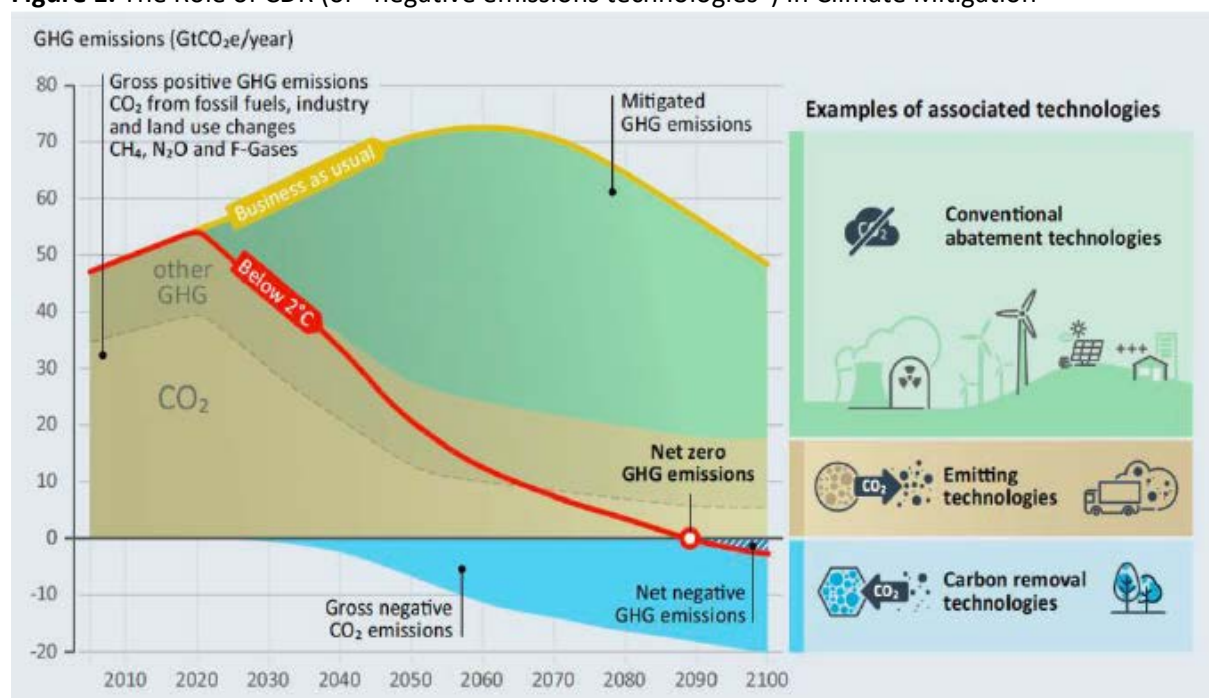
Figure 1. The Role of CDR (or “negative emissions technologies”) In Climate Mitigation 5
